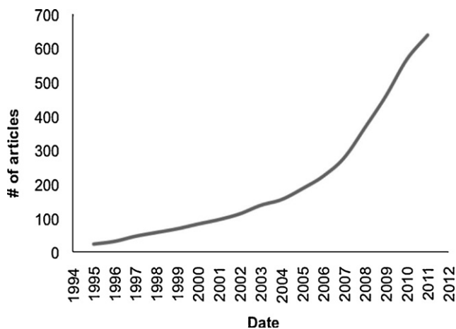
Fig. 1. Cumulative number of articles related to climate change impacts and biodiversity conservation (web of science search June 9, 2011). Search terms: climate SAME impact AND (species OR ecosystem OR biodiversity OR conservation OR "protected area" OR ecological OR restoration) NOT (aerosol* OR agricultur* OR tourism OR health OR climatology OR NPP or productivity OR production OR palaeo* OR paleo* OR atmosphere* OR pleistocene or soci* OR holocene OR crop* OR disease OR metero*).
