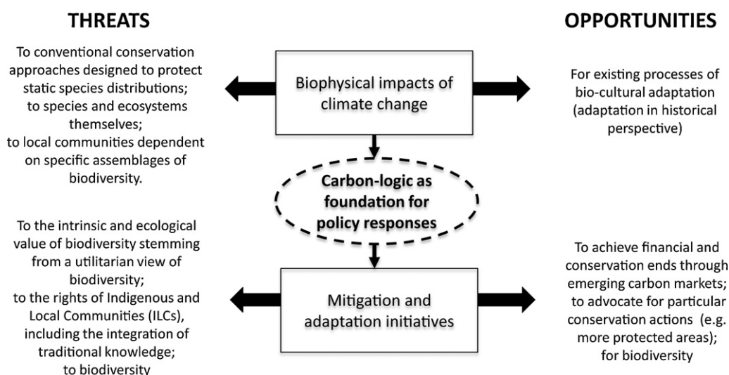
Fig. 2. Climate-Motivated Responses at COP 10 to the CBD.
